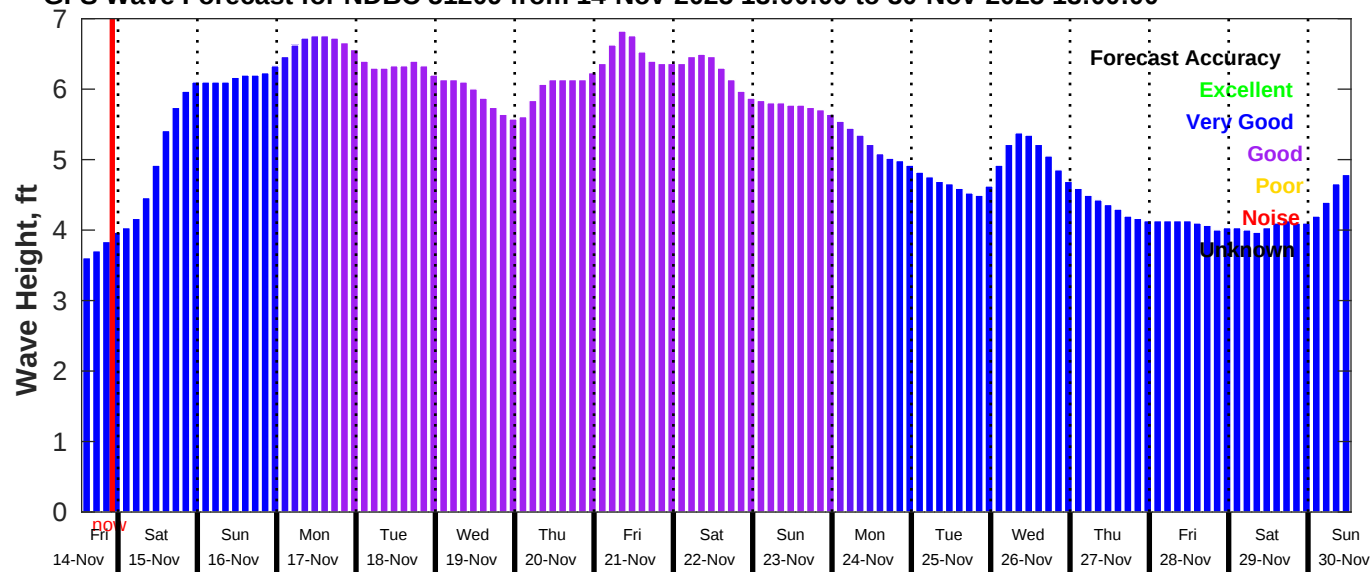
GFS Wave Forecast for NDBC 51209 from 14-Nov-2025 13:00:00 to 30-Nov-2025 13:00:00
