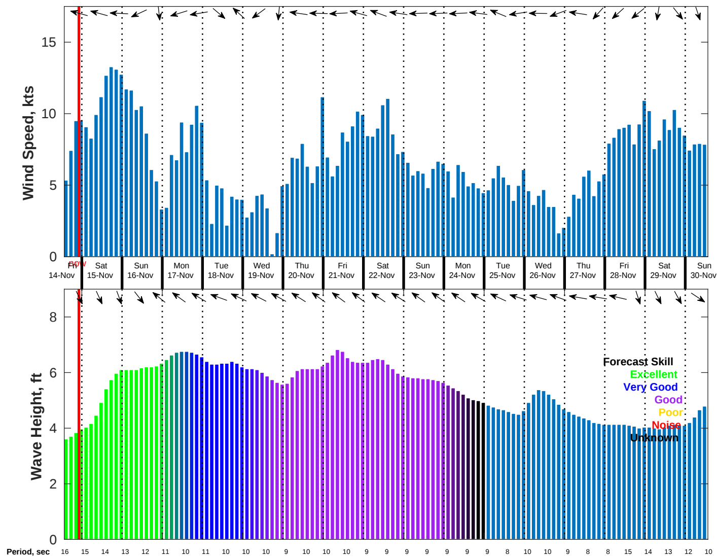
Wind & Wave Forecast for NDBC 51209 from 14-Nov-2025 13:00:00 to 30-Nov-2025 13:00:00
