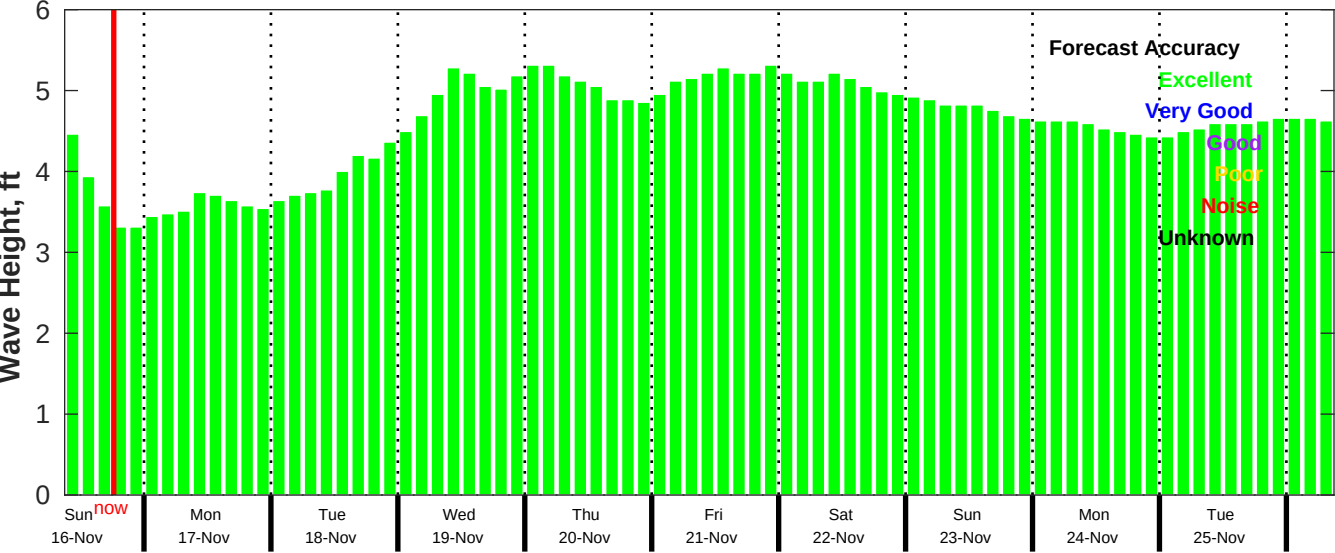
CMEMS Wave Forecast for NDBC 52212 from 15-Nov-2025 09:00:00 to 25-Nov-2025 09:00:00
