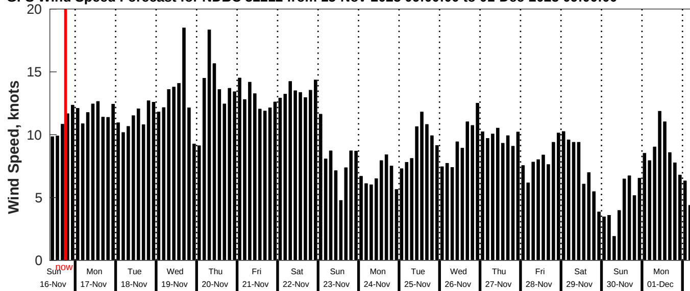
GFS Wind Speed Forecast for NDBC 52212 from 15-Nov-2025 09:00:00 to 01-Dec-2025 09:00:00
