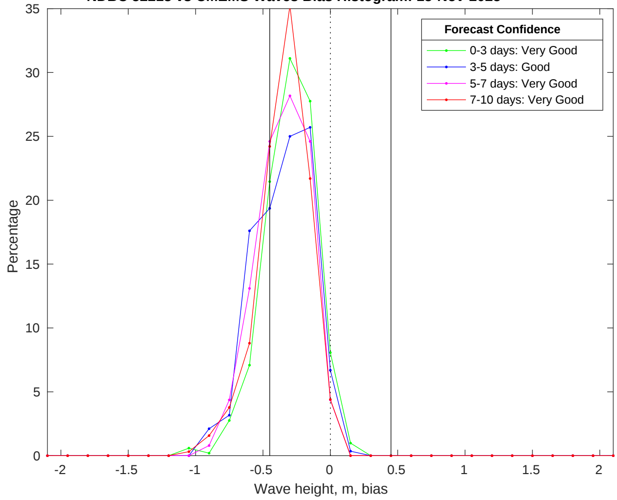
NDBC 52213 vs CMEMS Waves Bias Histogram: 15-Nov-2025
