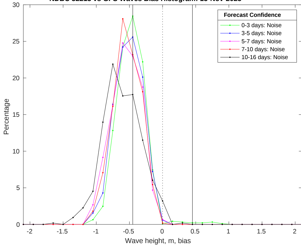
NDBC 52213 vs GFS Waves Bias Histogram: 15-Nov-2025
