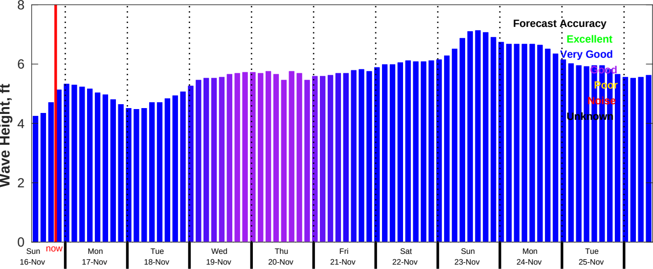
CMEMS Wave Forecast for NDBC 52213 from 15-Nov-2025 11:00:00 to 25-Nov-2025 11:00:00
