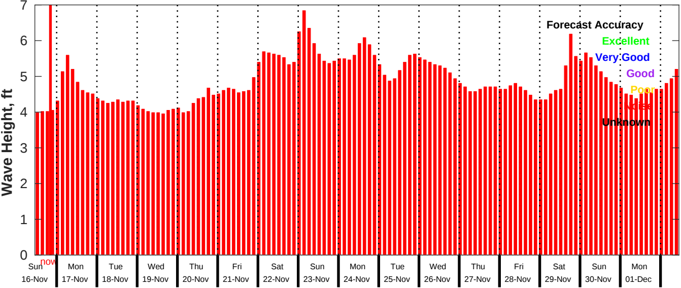
GFS Wave Forecast for NDBC 52213 from 15-Nov-2025 11:00:00 to 01-Dec-2025 11:00:00
