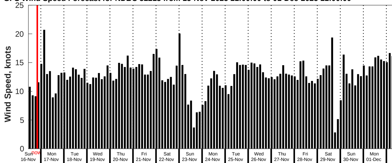
GFS Wind Speed Forecast for NDBC 52213 from 15-Nov-2025 11:00:00 to 01-Dec-2025 11:00:00
