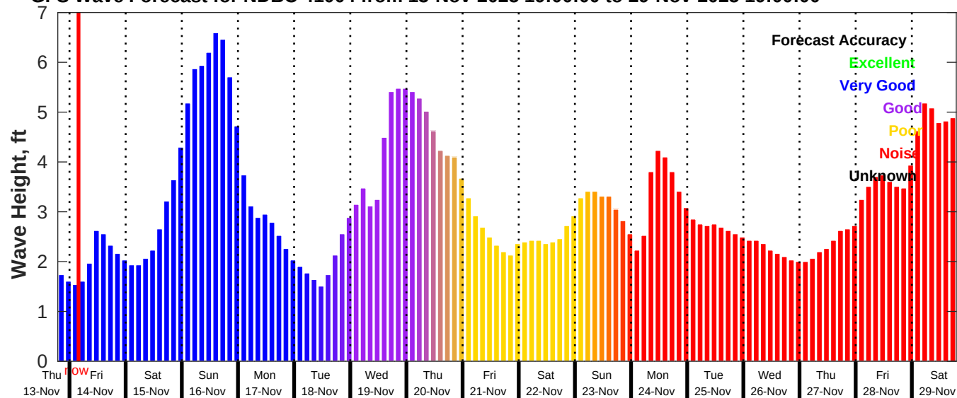
GFS Wave Forecast for NDBC 41004 from 13-Nov-2025 19:00:00 to 29-Nov-2025 19:00:00
