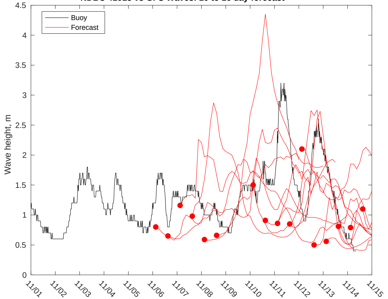
NDBC 41013 vs GFS Waves: 10 to 16 day forecast
