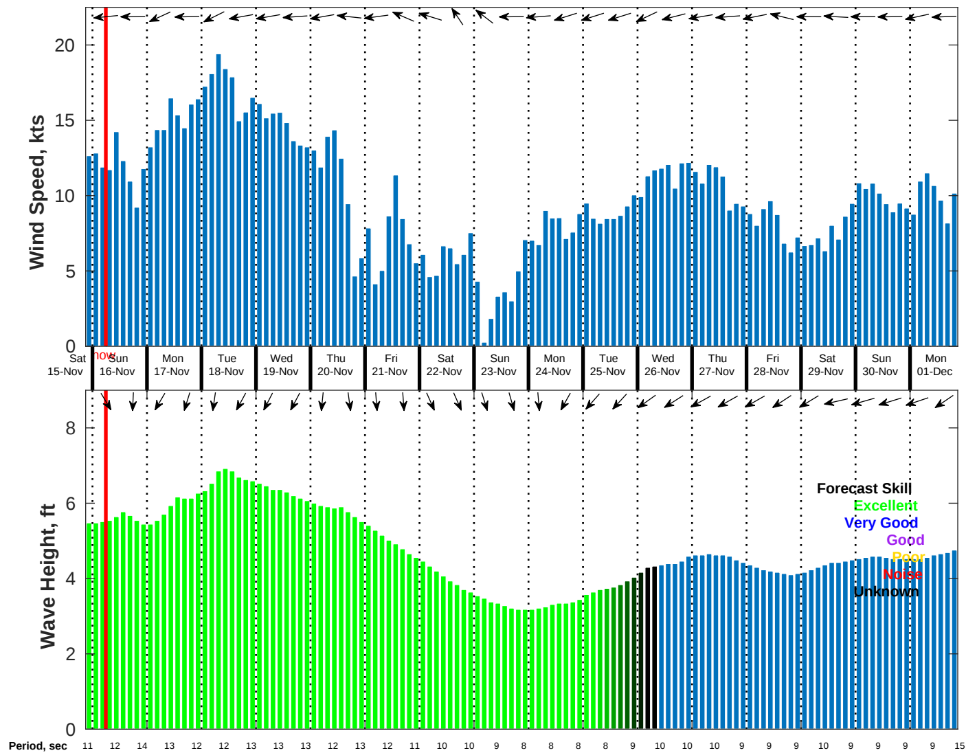
Wind & Wave Forecast for NDBC 41040 from 15-Nov-2025 21:00:00 to 01-Dec-2025 21:00:00
