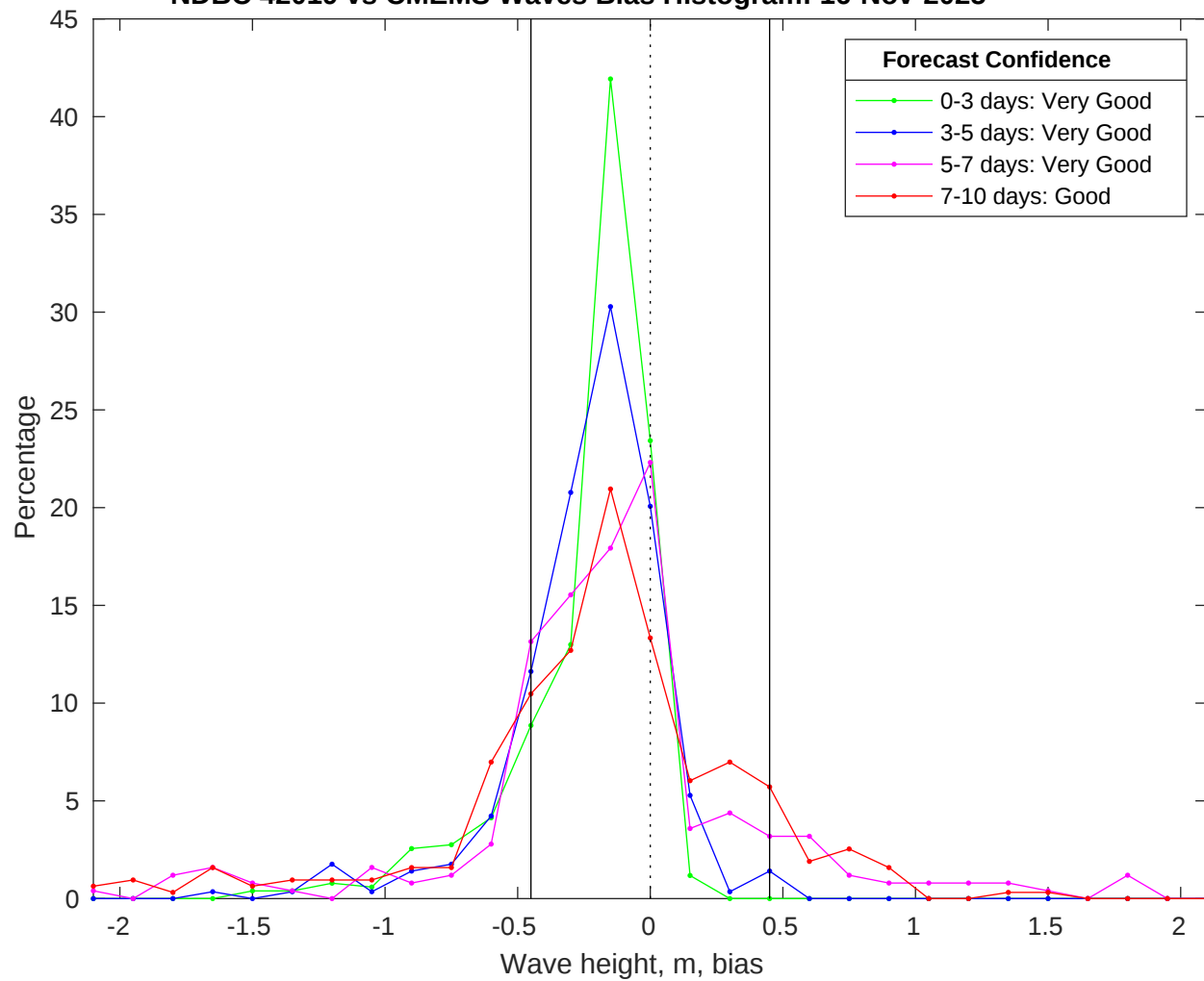
NDBC 42019 vs CMEMS Waves Bias Histogram: 16-Nov-2025
