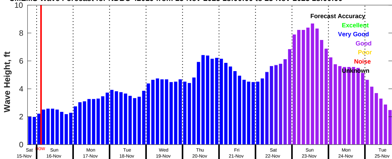
CMEMS Wave Forecast for NDBC 42019 from 15-Nov-2025 18:00:00 to 25-Nov-2025 18:00:00
