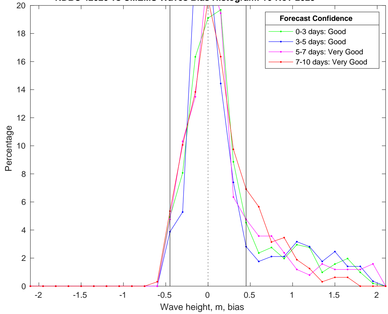
NDBC 42020 vs CMEMS Waves Bias Histogram: 16-Nov-2025
