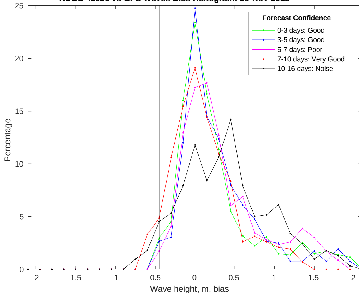
NDBC 42020 vs GFS Waves Bias Histogram: 16-Nov-2025
