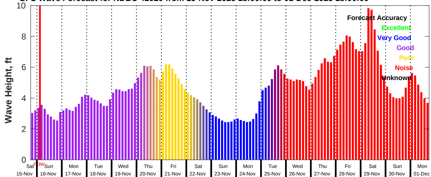
GFS Wave Forecast for NDBC 42020 from 15-Nov-2025 18:00:00 to 01-Dec-2025 18:00:00
