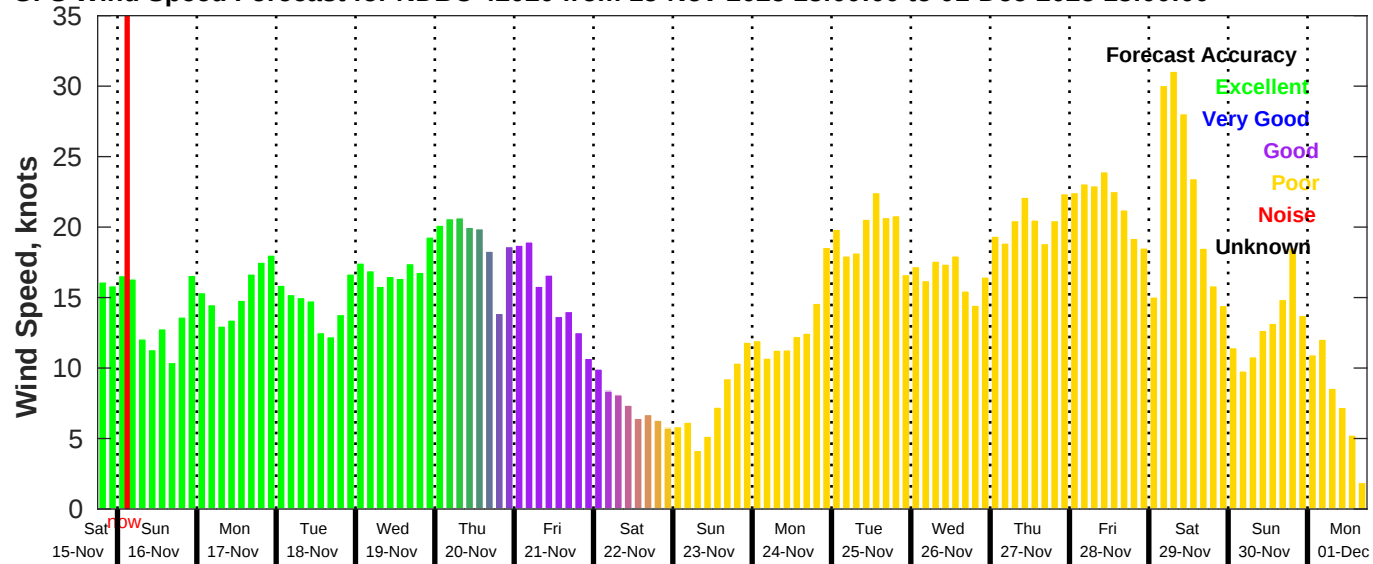
GFS Wind Speed Forecast for NDBC 42020 from 15-Nov-2025 18:00:00 to 01-Dec-2025 18:00:00
