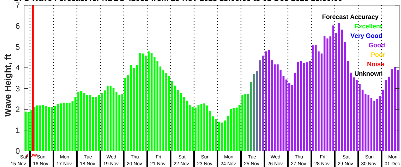
GFS Wave Forecast for NDBC 42035 from 15-Nov-2025 18:00:00 to 01-Dec-2025 18:00:00
