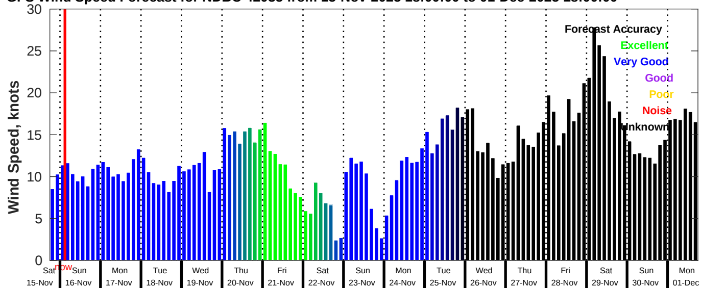
GFS Wind Speed Forecast for NDBC 42035 from 15-Nov-2025 18:00:00 to 01-Dec-2025 18:00:00
