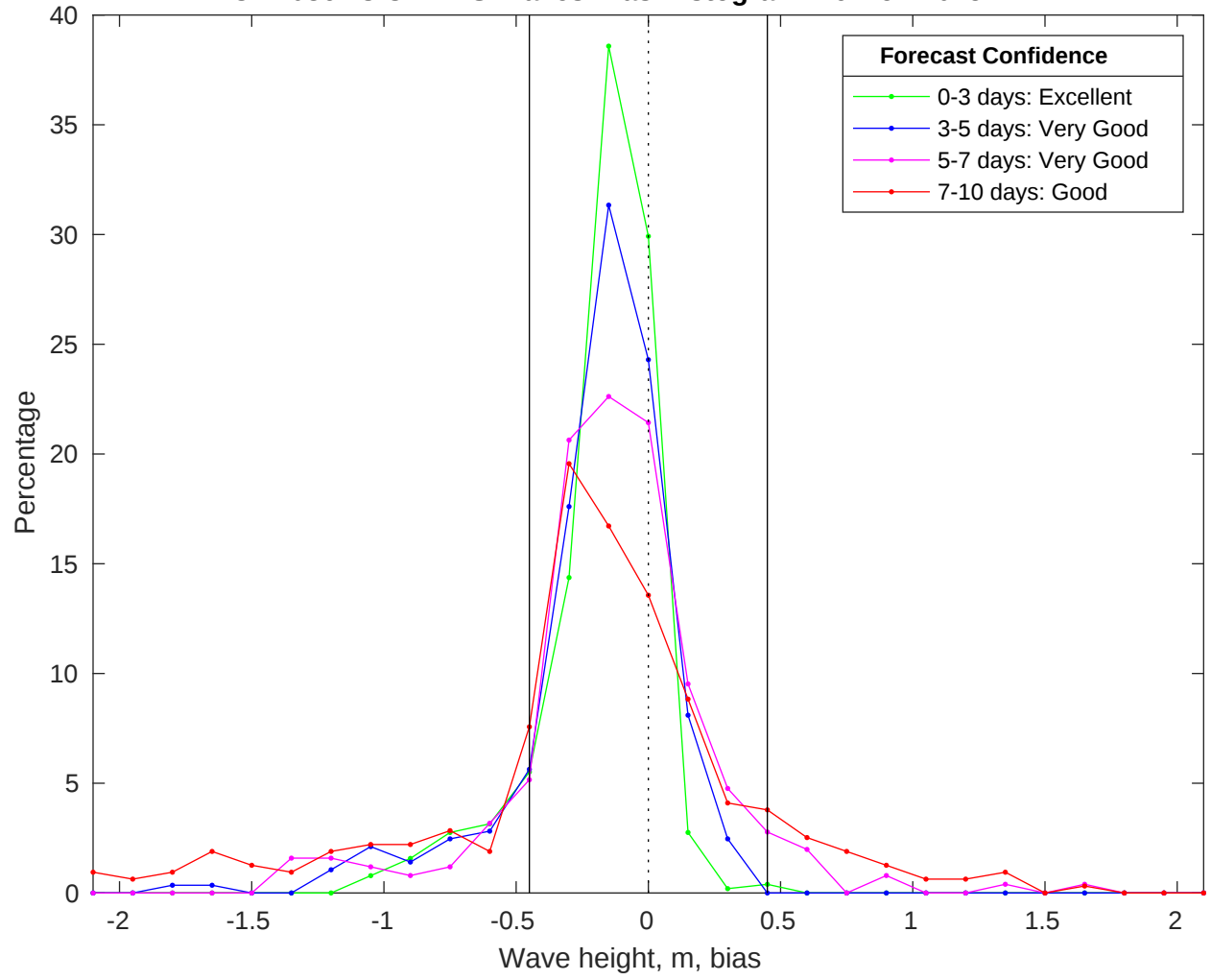
NDBC 42036 vs CMEMS Waves Bias Histogram: 16-Nov-2025
