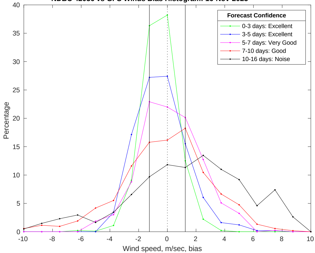
NDBC 42036 vs GFS Winds Bias Histogram: 16-Nov-2025
