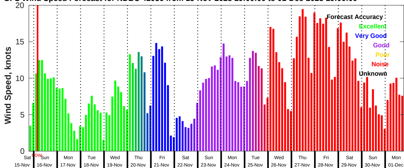
GFS Wind Speed Forecast for NDBC 42036 from 15-Nov-2025 19:00:00 to 01-Dec-2025 19:00:00
