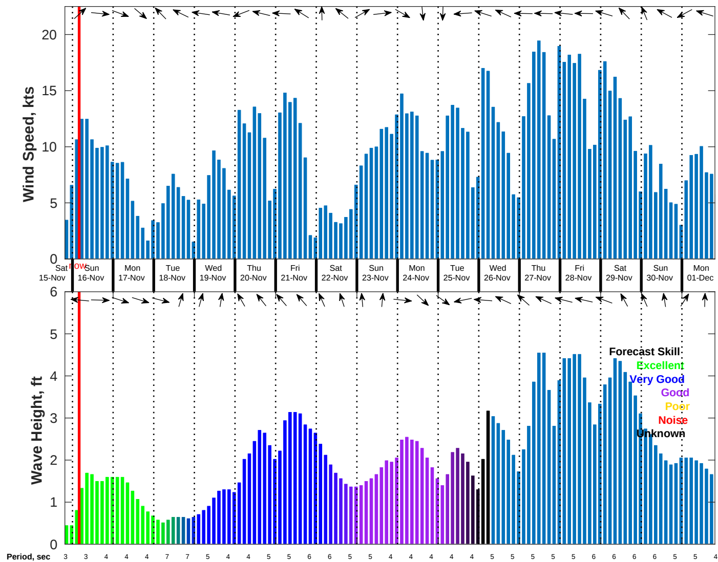
Wind & Wave Forecast for NDBC 42036 from 15-Nov-2025 19:00:00 to 01-Dec-2025 19:00:00
