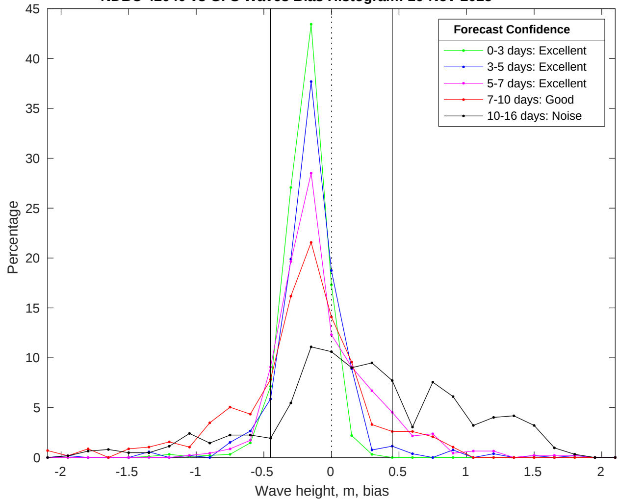
NDBC 42040 vs GFS Waves Bias Histogram: 16-Nov-2025
