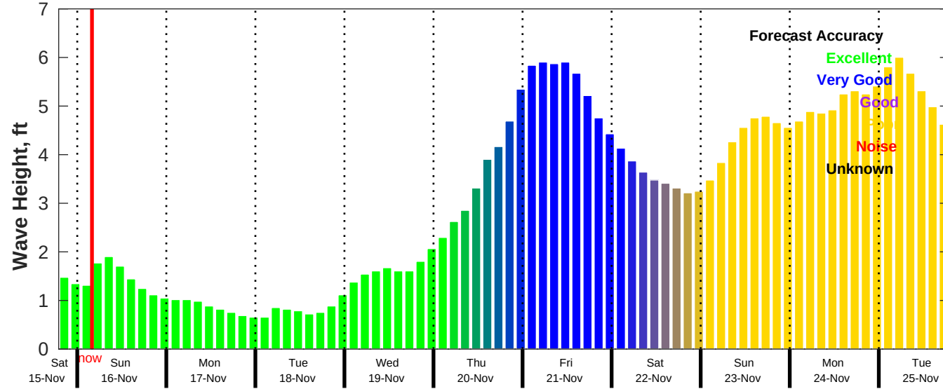
CMEMS Wave Forecast for NDBC 42040 from 15-Nov-2025 19:00:00 to 25-Nov-2025 19:00:00
