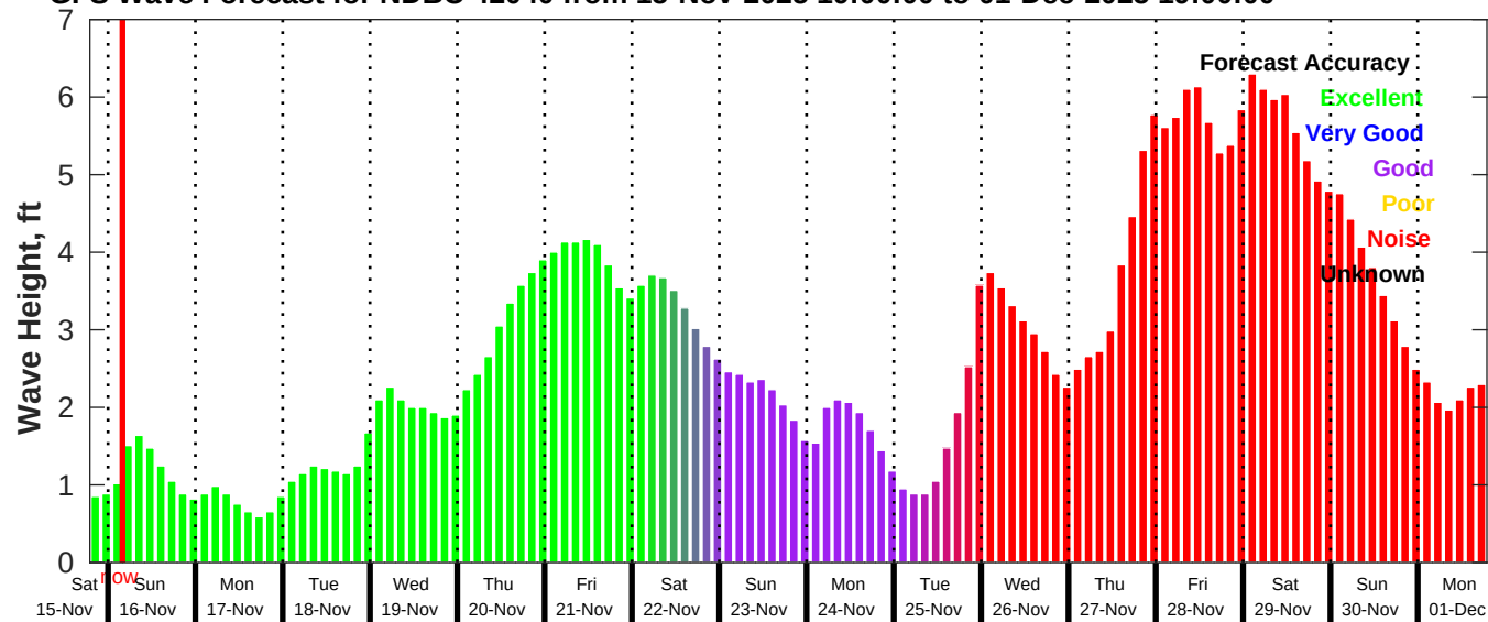
GFS Wave Forecast for NDBC 42040 from 15-Nov-2025 19:00:00 to 01-Dec-2025 19:00:00
