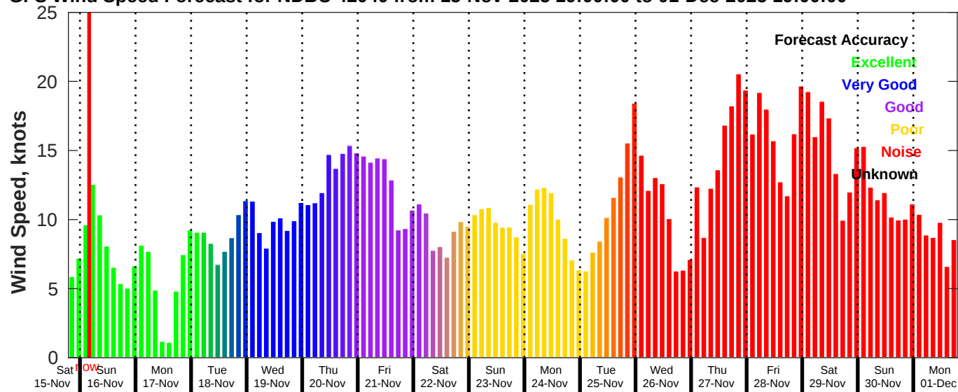
GFS Wind Speed Forecast for NDBC 42040 from 15-Nov-2025 19:00:00 to 01-Dec-2025 19:00:00
