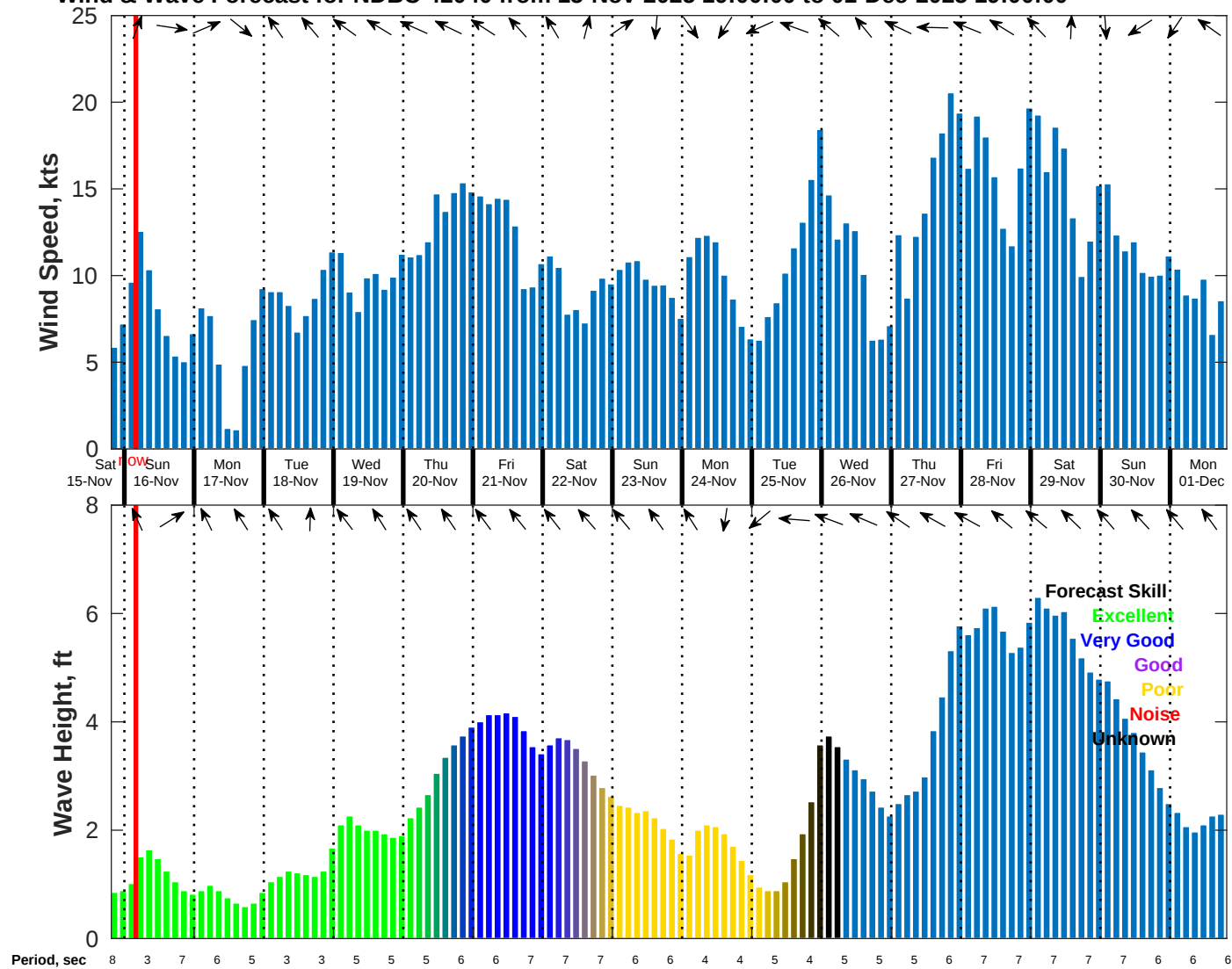
Wind & Wave Forecast for NDBC 42040 from 15-Nov-2025 19:00:00 to 01-Dec-2025 19:00:00
