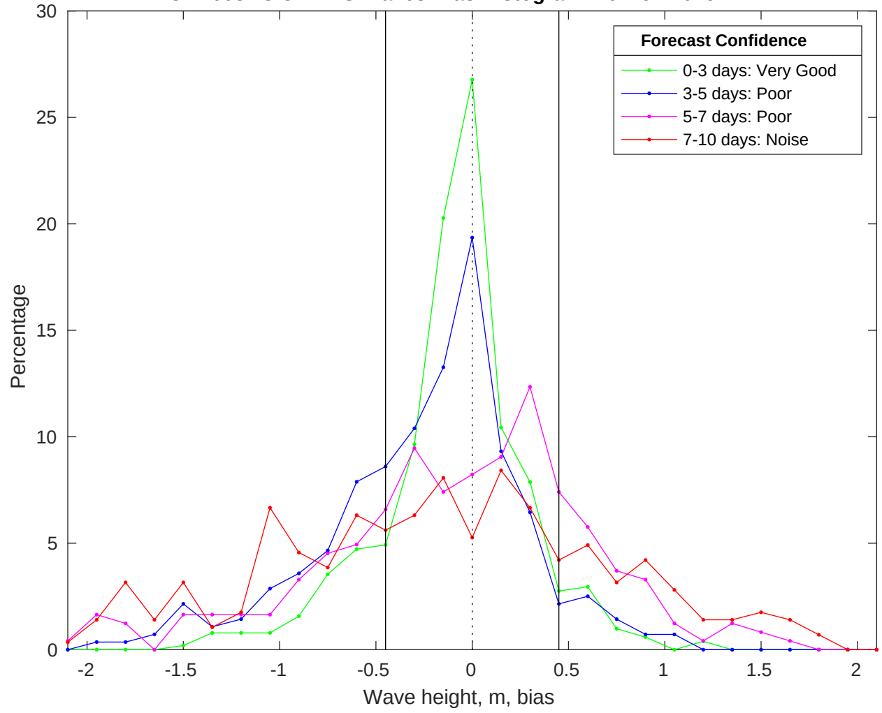
NDBC 44008 vs CMEMS Waves Bias Histogram: 16-Nov-2025
