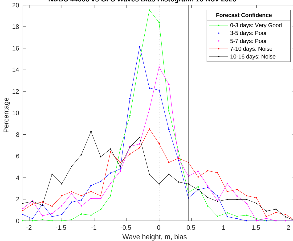
NDBC 44008 vs GFS Waves Bias Histogram: 16-Nov-2025
