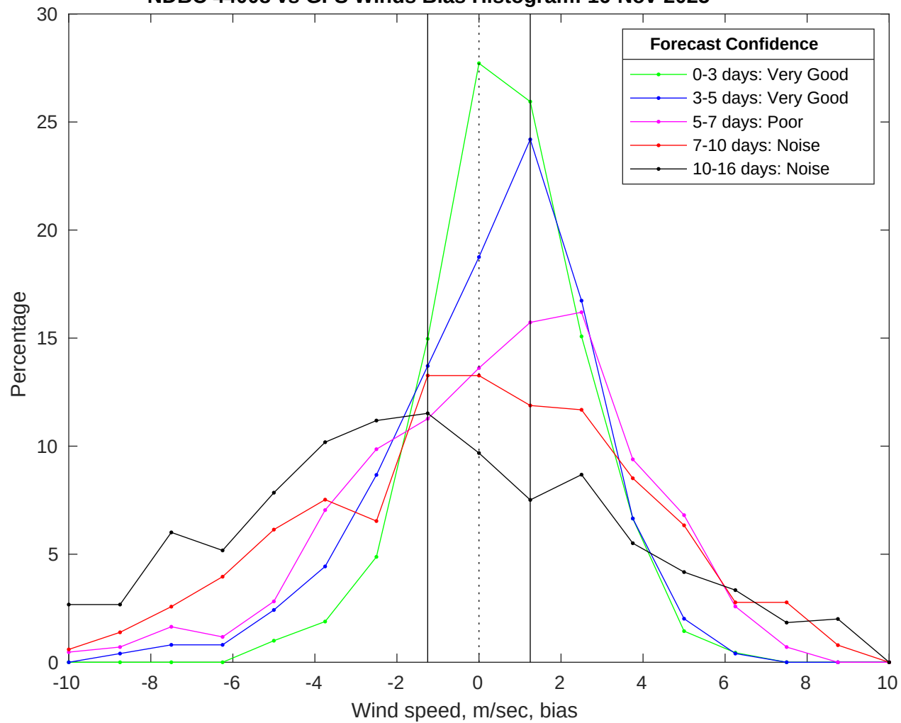
NDBC 44008 vs GFS Winds Bias Histogram: 16-Nov-2025
