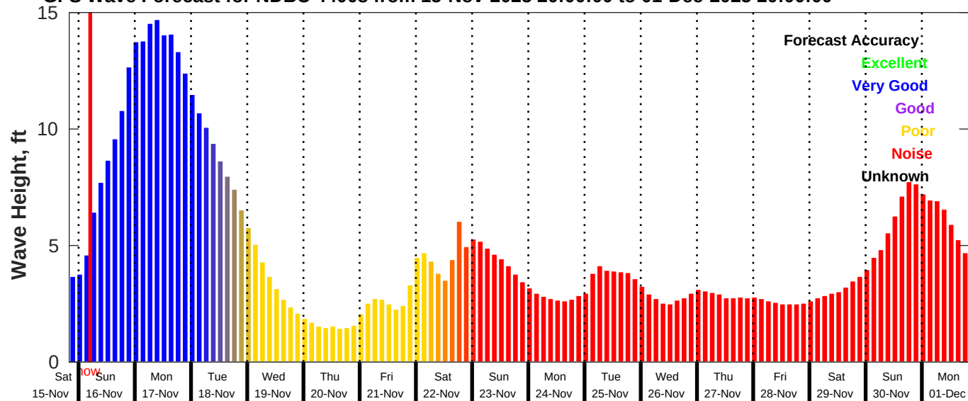
GFS Wave Forecast for NDBC 44008 from 15-Nov-2025 20:00:00 to 01-Dec-2025 20:00:00
