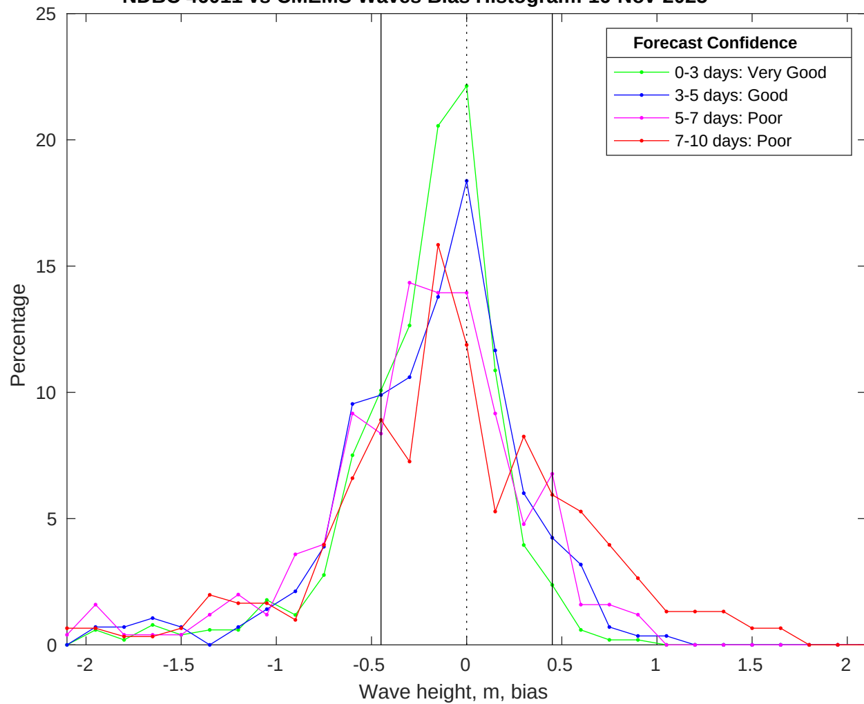
NDBC 46011 vs CMEMS Waves Bias Histogram: 16-Nov-2025
