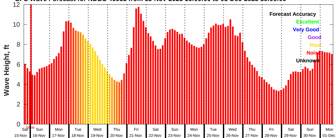
GFS Wave Forecast for NDBC 46011 from 15-Nov-2025 16:00:00 to 01-Dec-2025 16:00:00
