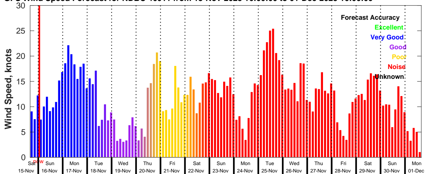
GFS Wind Speed Forecast for NDBC 46011 from 15-Nov-2025 16:00:00 to 01-Dec-2025 16:00:00
