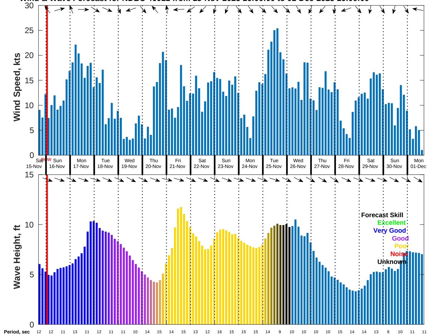
Wind & Wave Forecast for NDBC 46011 from 15-Nov-2025 16:00:00 to 01-Dec-2025 16:00:00
