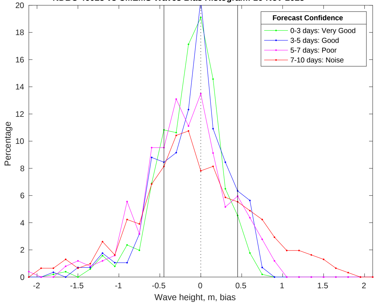
NDBC 46028 vs CMEMS Waves Bias Histogram: 16-Nov-2025
