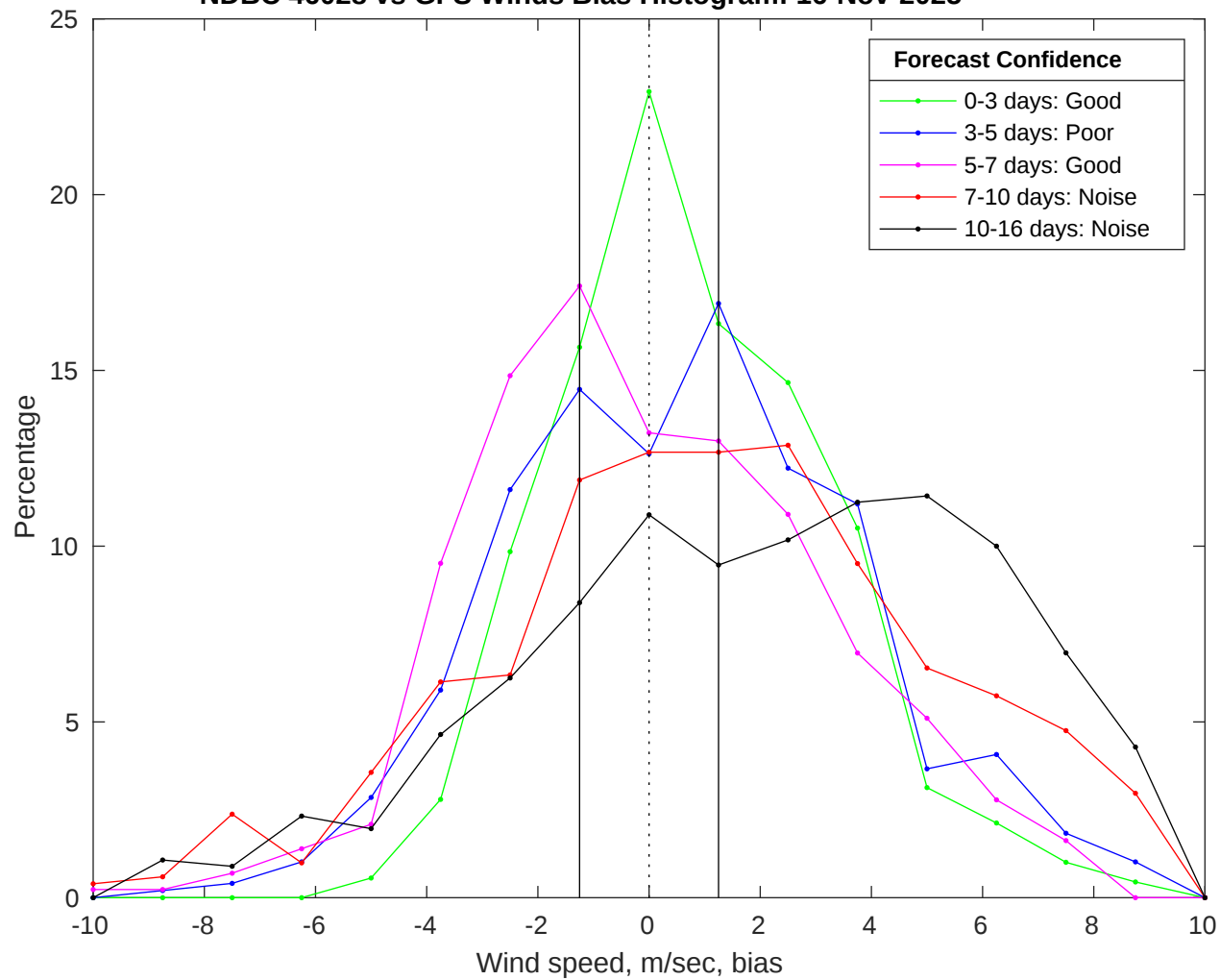
NDBC 46028 vs GFS Winds Bias Histogram: 16-Nov-2025
