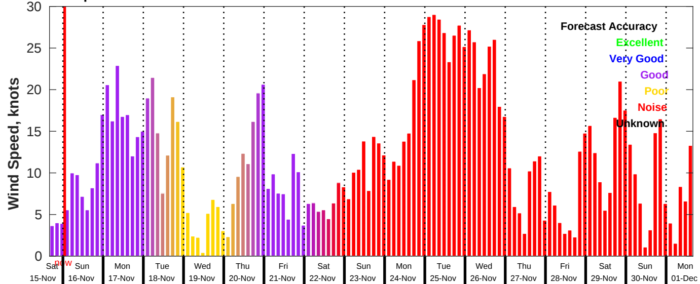
GFS Wind Speed Forecast for NDBC 46028 from 15-Nov-2025 16:00:00 to 01-Dec-2025 16:00:00
