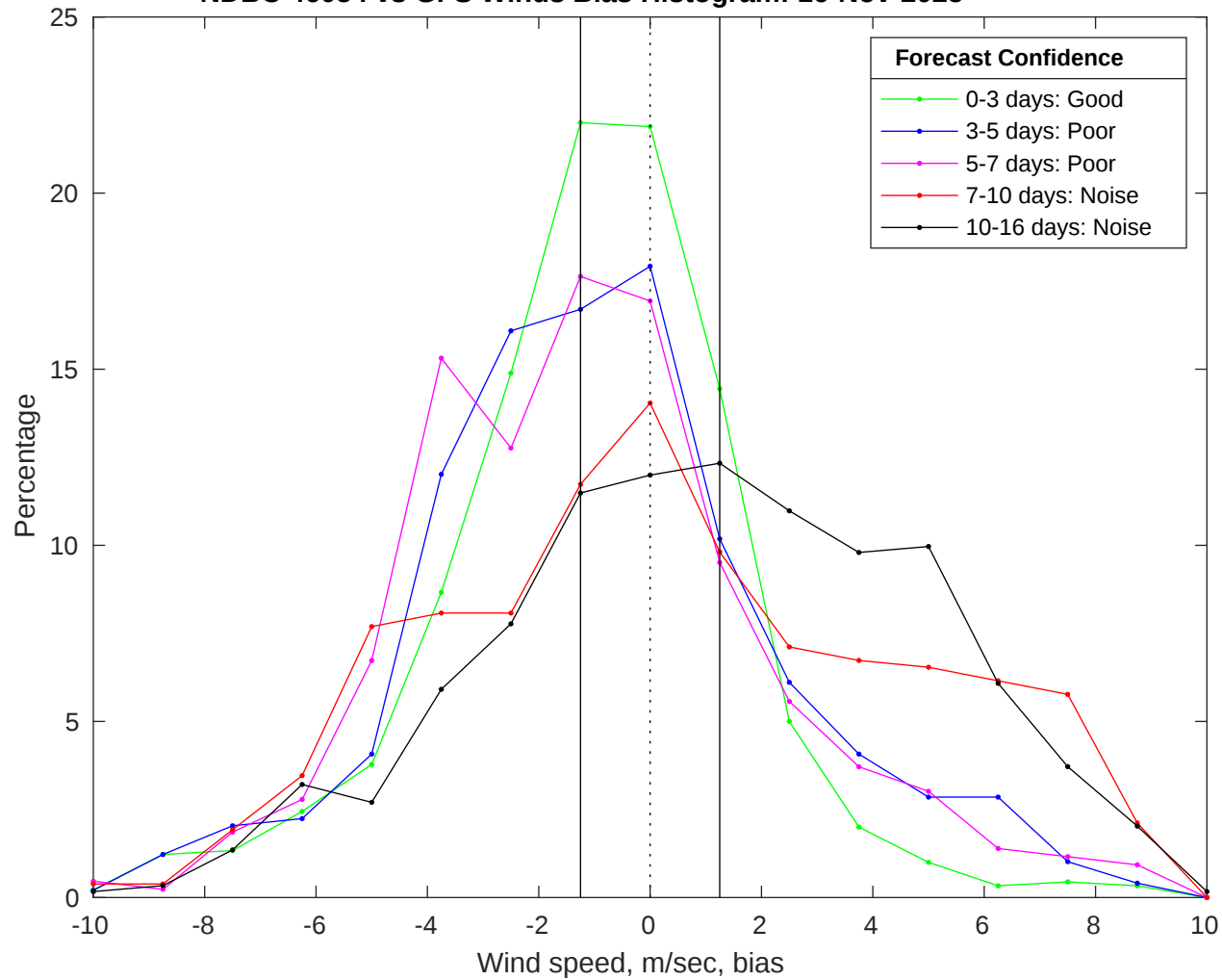
NDBC 46054 vs GFS Winds Bias Histogram: 16-Nov-2025
