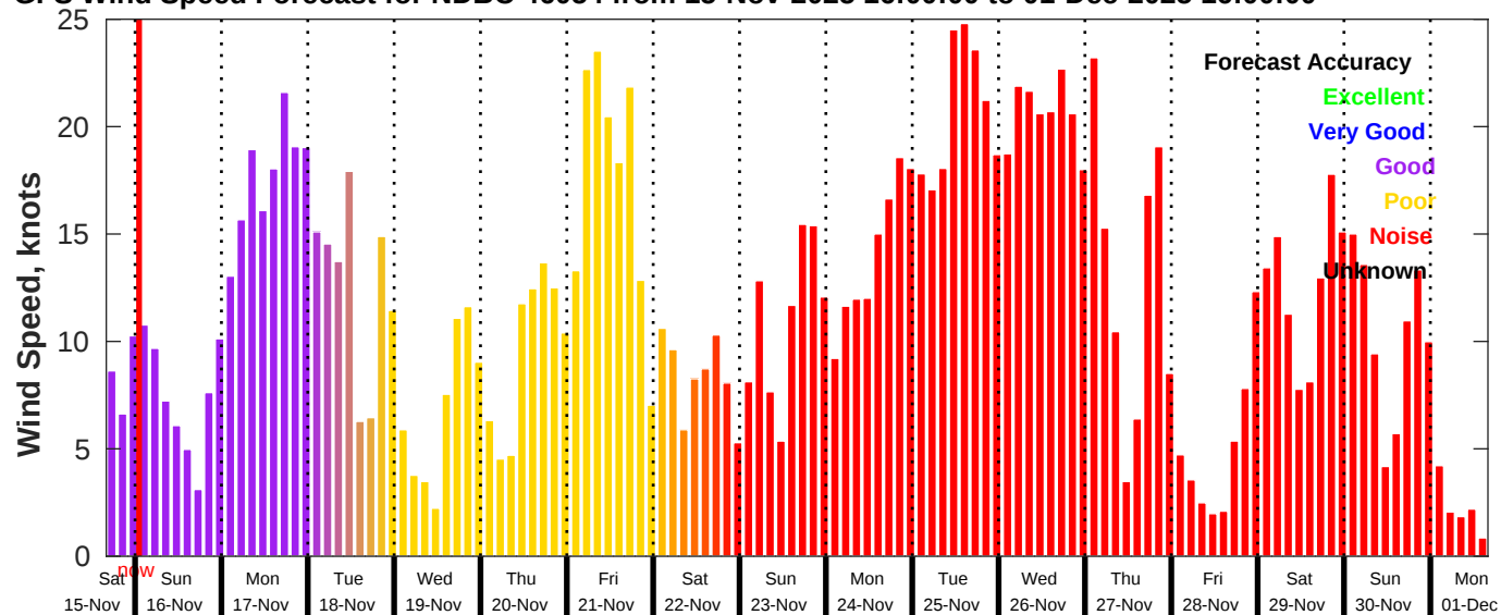
GFS Wind Speed Forecast for NDBC 46054 from 15-Nov-2025 16:00:00 to 01-Dec-2025 16:00:00
