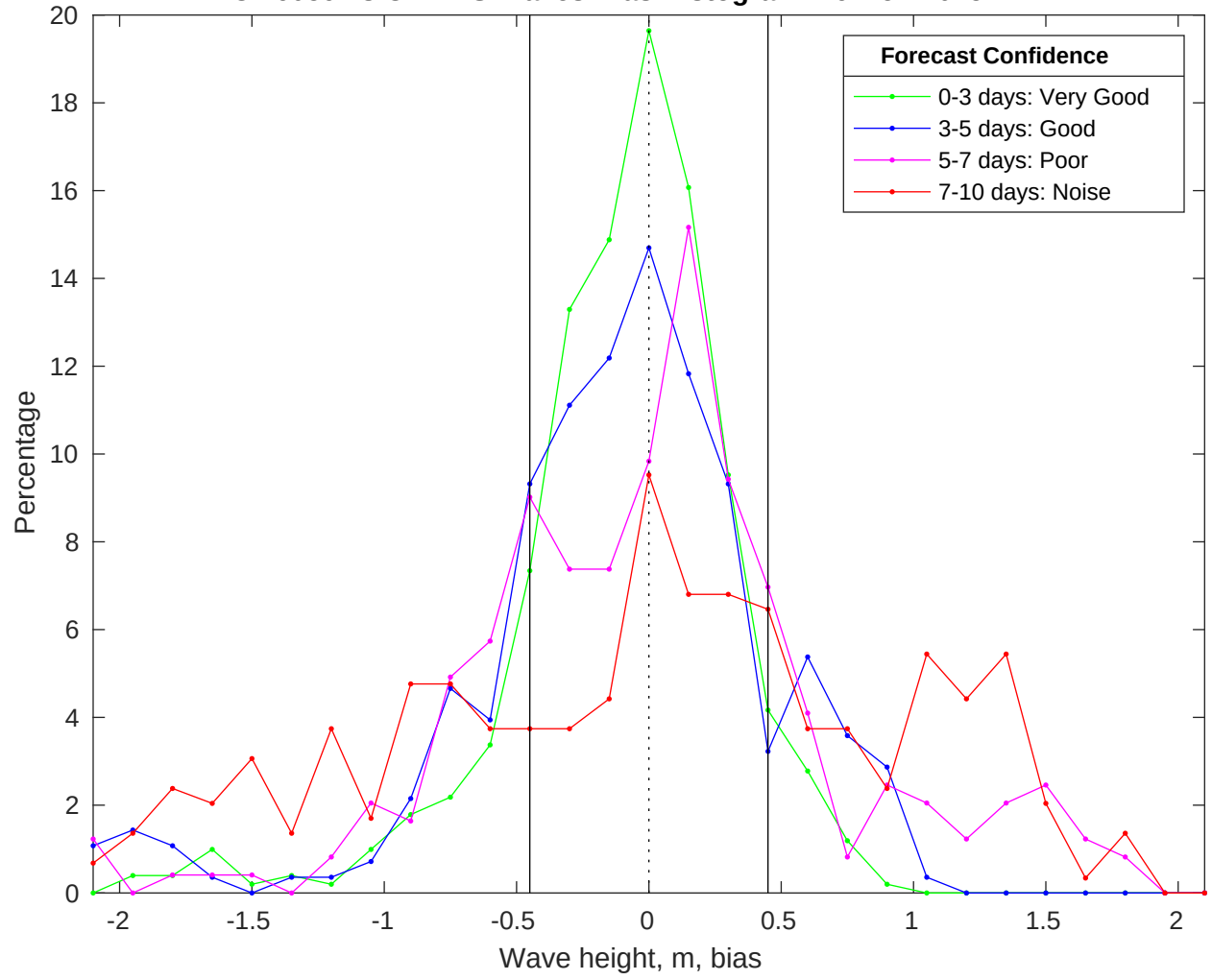
NDBC 46059 vs CMEMS Waves Bias Histogram: 16-Nov-2025
