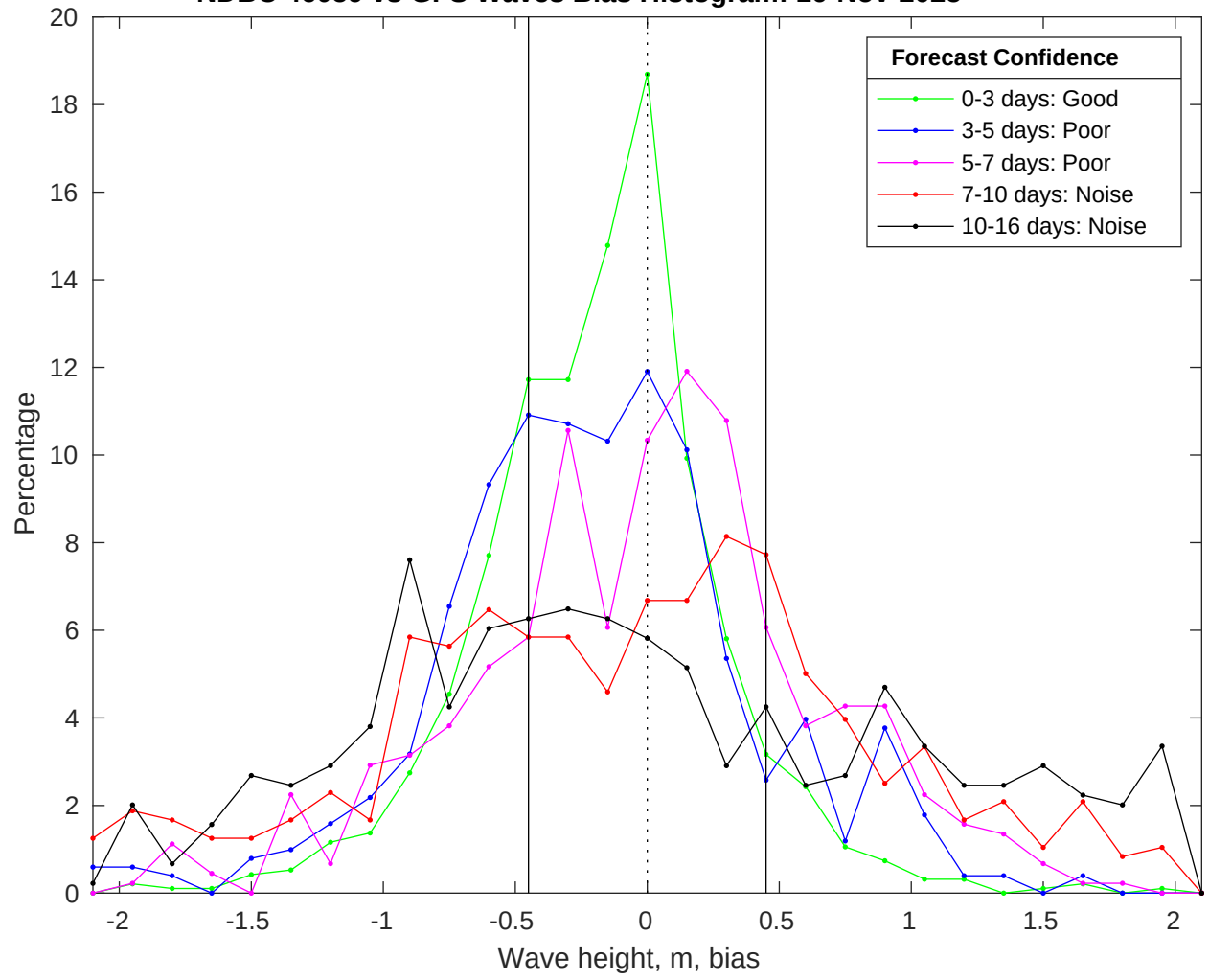
NDBC 46059 vs GFS Waves Bias Histogram: 16-Nov-2025
