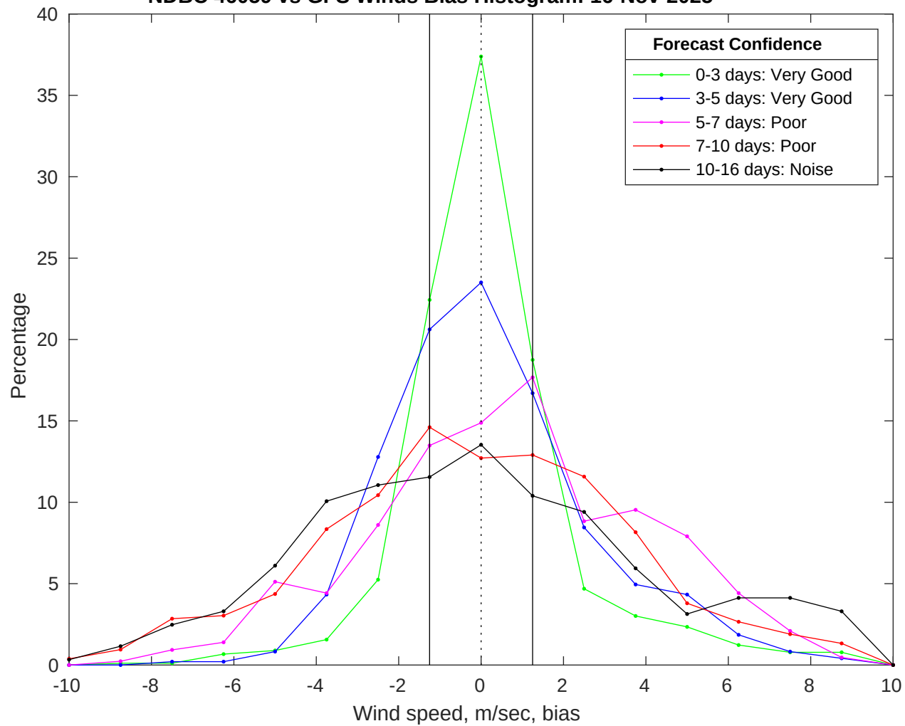
NDBC 46059 vs GFS Winds Bias Histogram: 16-Nov-2025
