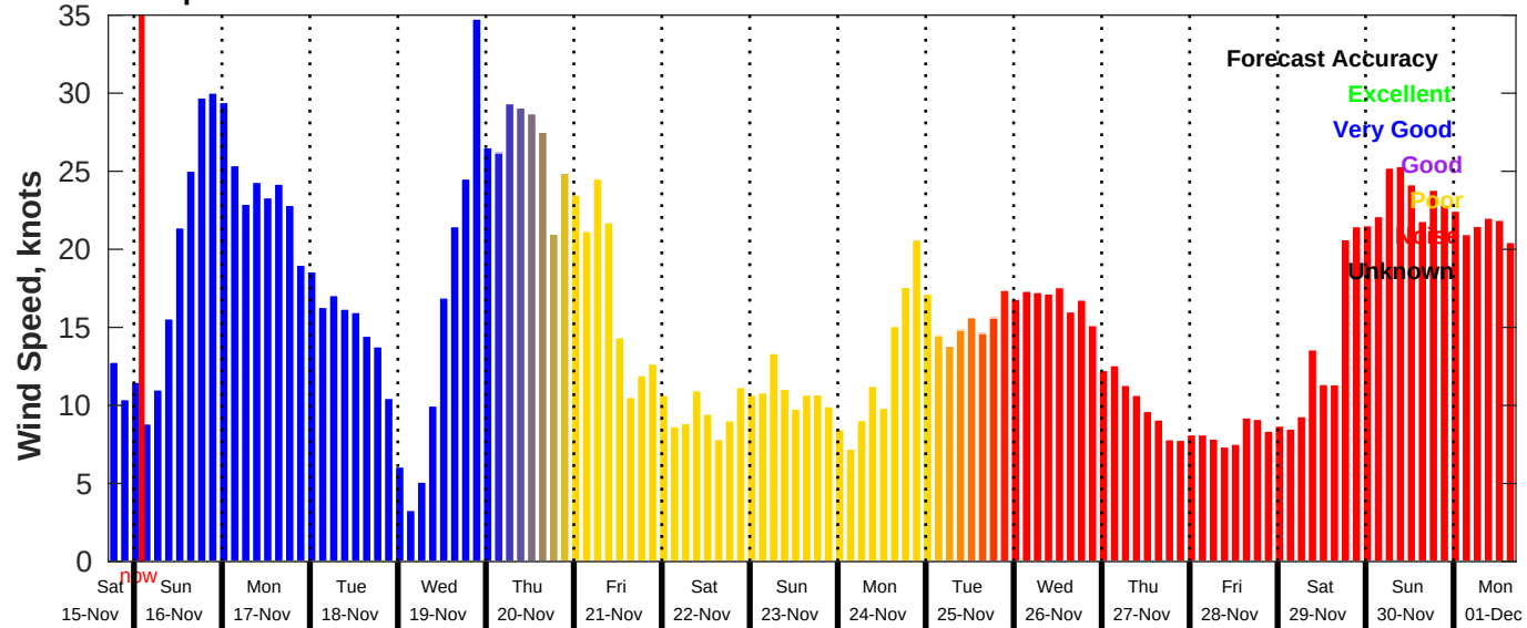
GFS Wind Speed Forecast for NDBC 46059 from 15-Nov-2025 17:00:00 to 01-Dec-2025 17:00:00
