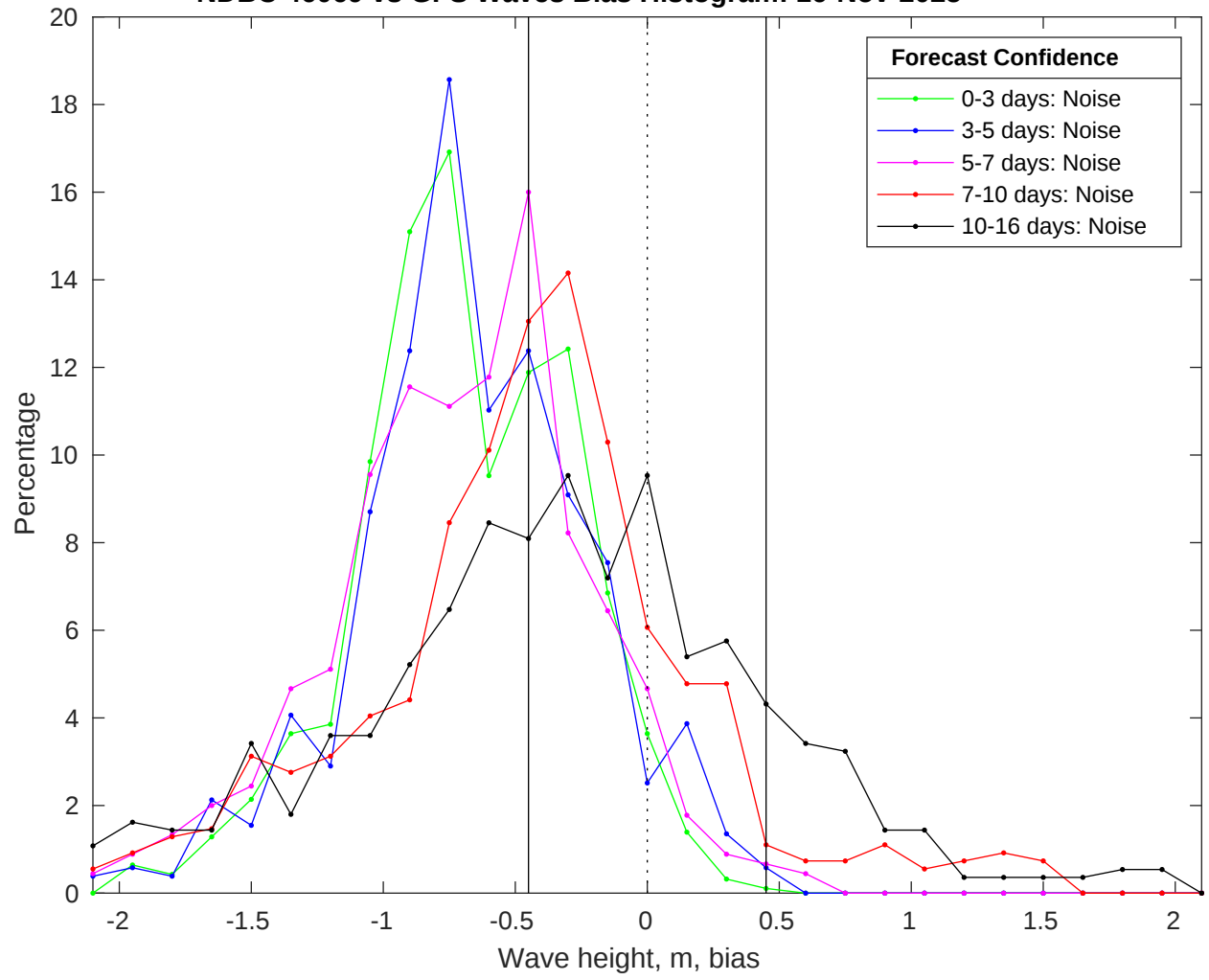
NDBC 46069 vs GFS Waves Bias Histogram: 16-Nov-2025
