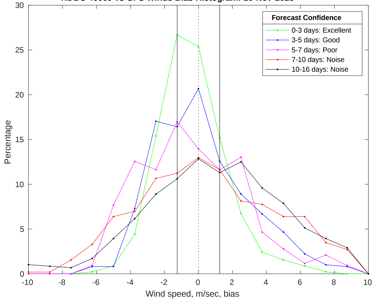
NDBC 46069 vs GFS Winds Bias Histogram: 16-Nov-2025
