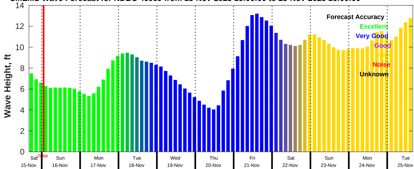
CMEMS Wave Forecast for NDBC 46069 from 15-Nov-2025 16:00:00 to 25-Nov-2025 16:00:00
