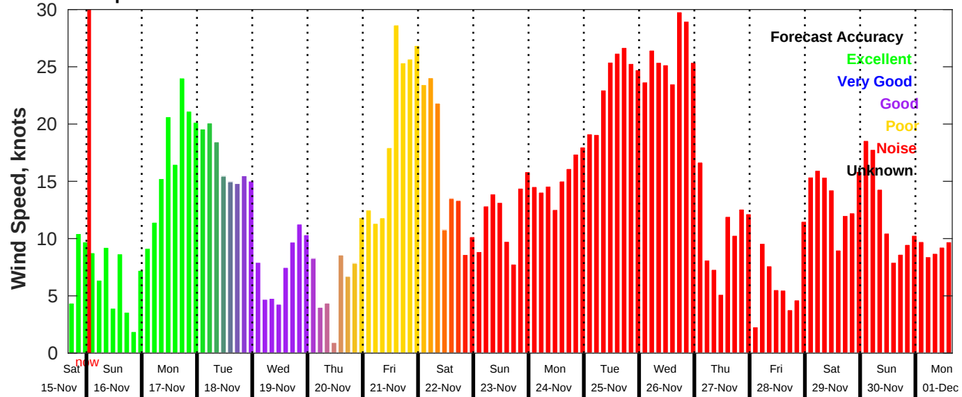
GFS Wind Speed Forecast for NDBC 46069 from 15-Nov-2025 16:00:00 to 01-Dec-2025 16:00:00
